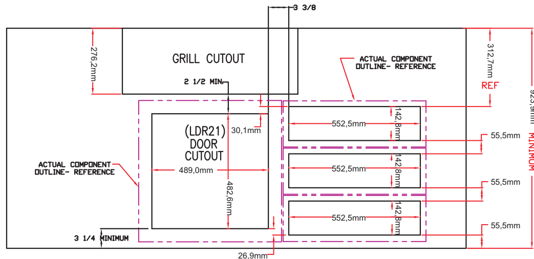
TYPICAL 1 OR 2-CLUSTER MOUNT DRAWER- INDEPENDENT FROM LDR
