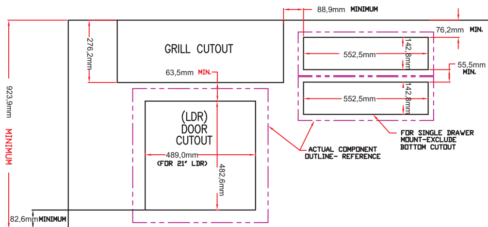
TYPICAL 1 OR 2-CLUSTER MOUNT DRAWER- INDEPENDENT FROM LDR
